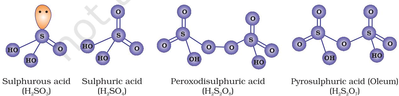
Fig. 7.6: Structures of some important oxoacids of sulphur
